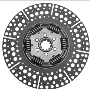
MB 1620 MODERNO SACHS 6 MOLAS 350MM
